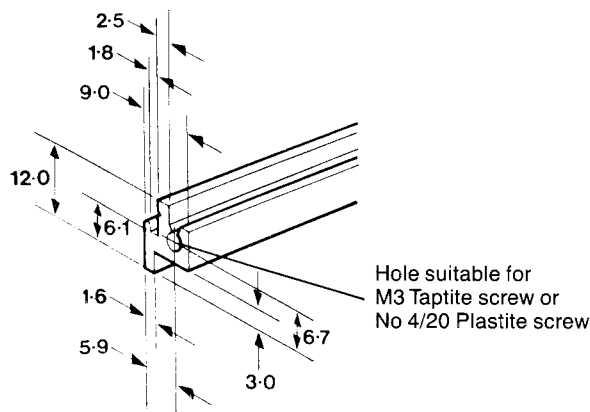
Flange Rail Profile
