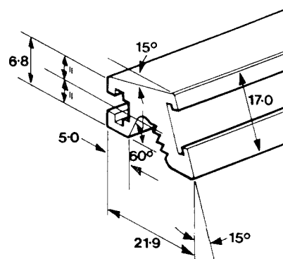
Handle Profile Series 2.
