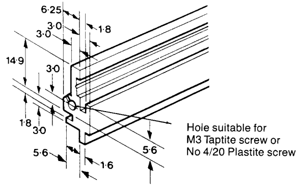
Single Flange Top Rail Profile used in Style 70 Unit Form
