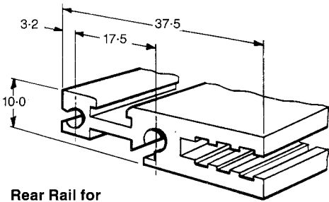
Rear Rail for Motherboard/Optional Connector Mounting Eurorack
