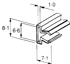
Designation retainer for TSR Subracks.
