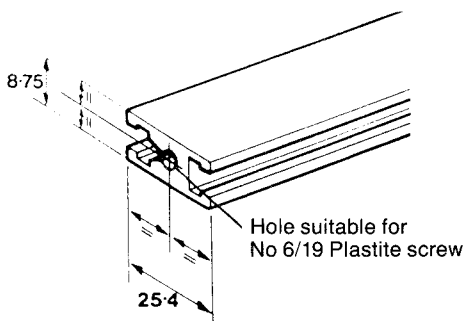
Connector Mounting Rail Profile Series 2
