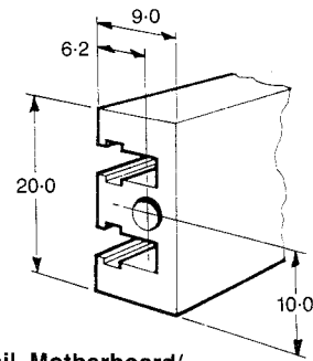
Centre Rail, Motherboard/ Optional Connector Mounting for 6U Eurorack
