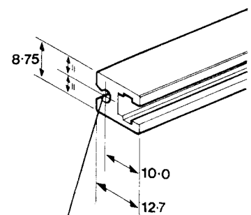
Connector Mounting Rail Profile Series 2
