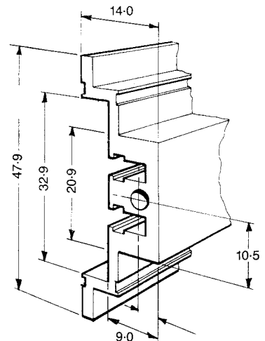
Centre Rail, Direct DIN Connector Mounting, for 6U Eurorack
