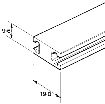
Horizontal Rail Profile used in TSR subracks
