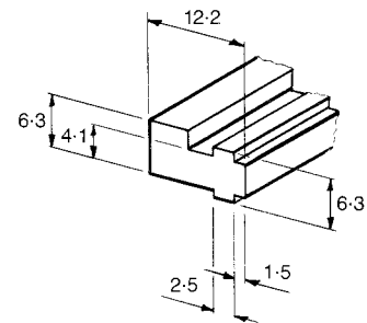
Trim strip for series 2.
