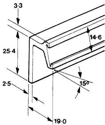
Handle Profile Style 70
