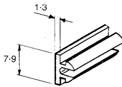
Designation strip for TSR Subracks.
