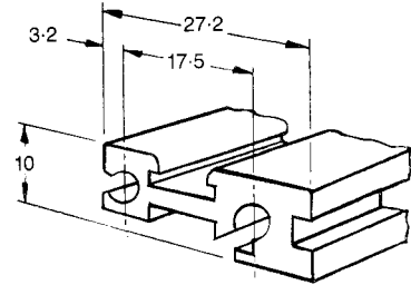
Rear Rail for Divided Eurorack
