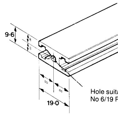
Horizontal Rail Profile used in TSR subracks
