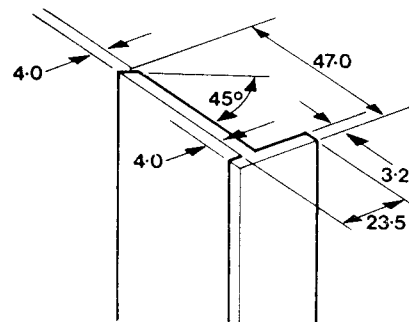
Front Mounting "T" Plate Profile Series 2
