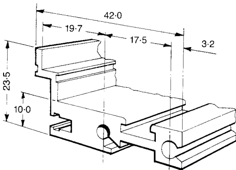
Rear Rail, Direct DIN Conector Mounting Eurorack
