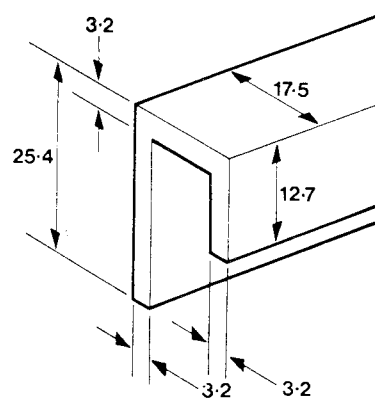
Handle Profile Style 19M
