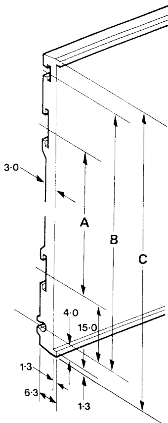
Front Panel Profile Style 70
