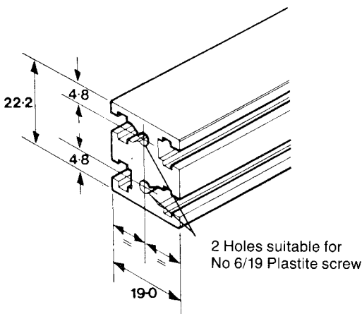
Double Horizontal Rail Profile
