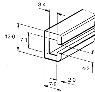
Handle profile.
