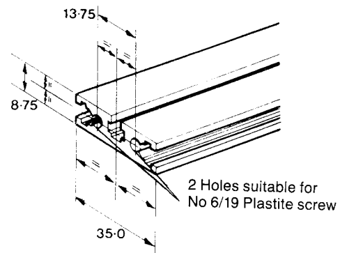
Horizontal Rail Profile Series 2
