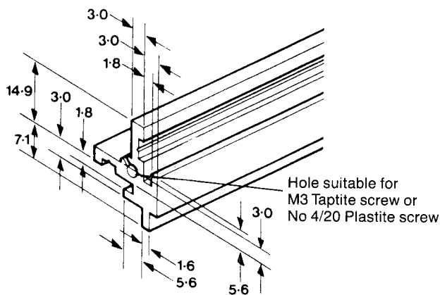
Double Flange Bottom Rail Profile used in Style 70 Unit Form
