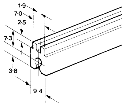
Guide Rail Profile for 1/16 in boards
