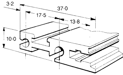
Front Rail and Rear Rail for Motherboard/Optional Connector Eurorack Mounting
