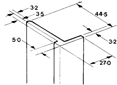
Front Mounting "T" Plate Profile used in TSR
